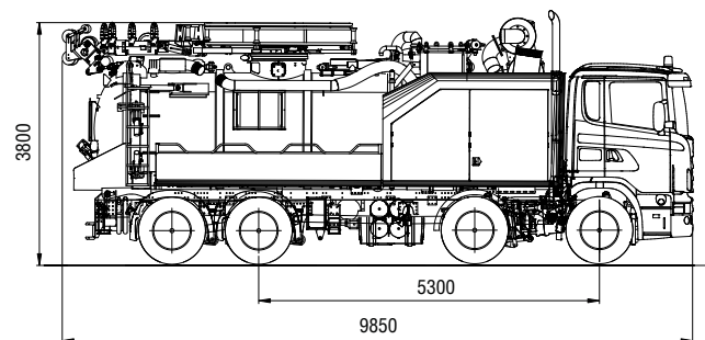
carcombi® FI 3200
