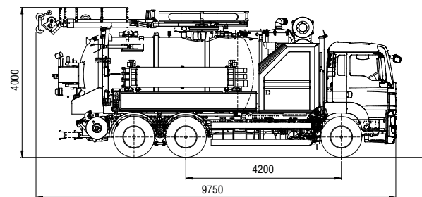
carcombi® FI 1800
