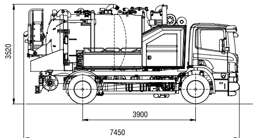
carcombi® FI 1800
