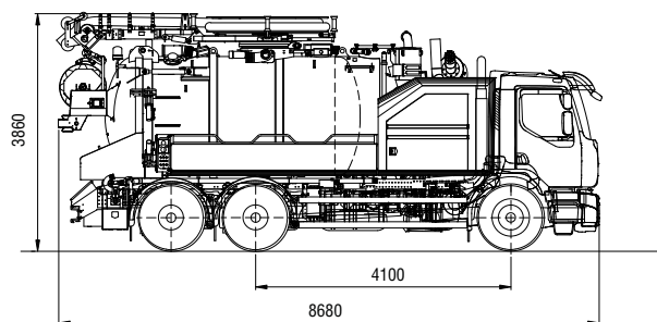
carcombi® FI 2600
